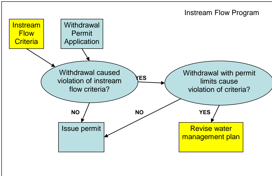
Figure 6. Use of Instream Flow Criteria to evaluate water withdrawal or reservoir release permits.
