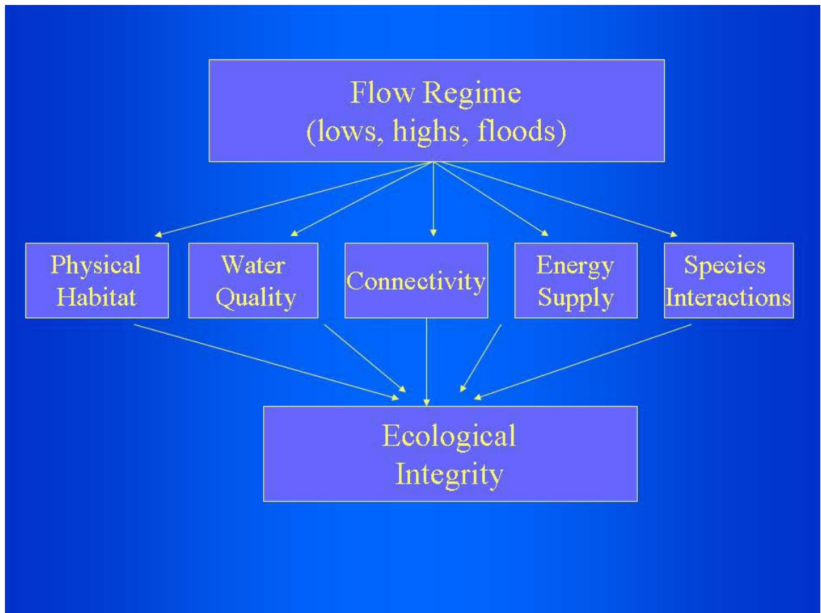
Figure 1. Relationship of flow regime to components of aquatic habitats. (Poff et al 1997, after Karr 1991)
